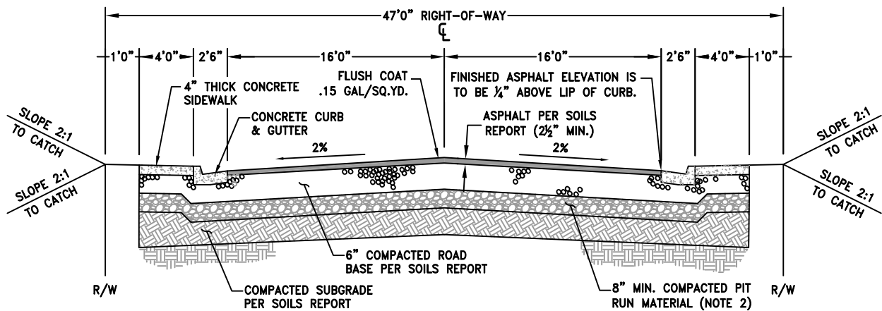
TYPICAL ROAD SECTION - 47'0" RIGHT-OF-WAY N.T.S.
