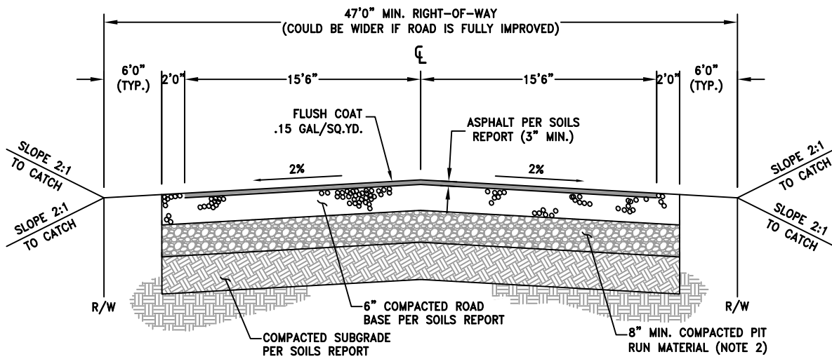
TYPICAL INDUSTRIAL ROAD SECTION - UNIMPROVED ROAD N.T.S.
