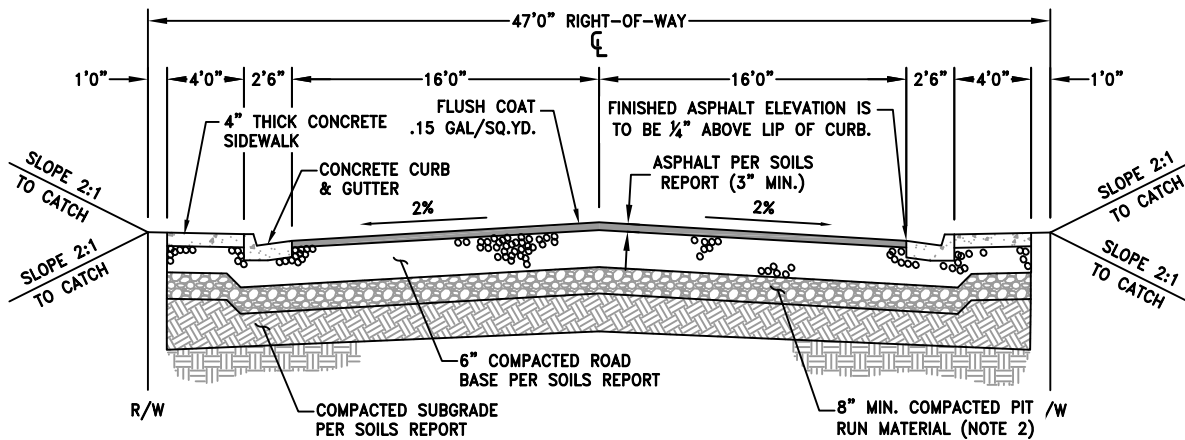
TYPICAL INDUSTRIAL ROAD SECTION - 47'0" RIGHT-OF-WAY N.T.S.
